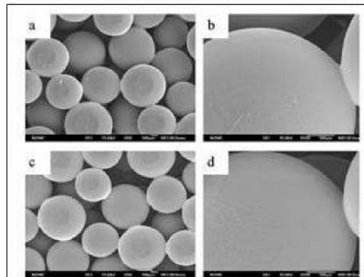
Fig 2B: Scanning electron micrographs indicating the effect of acetic acid treatment on the morphology of PLGA scaffolds. No obvious morphological change was observed on PLGA scaffold before (a and b) and after (c and d) acetic acid treatment. Magnification: X50 (a and c) and X 200 (b and d) (Jiang et al, 2010)
