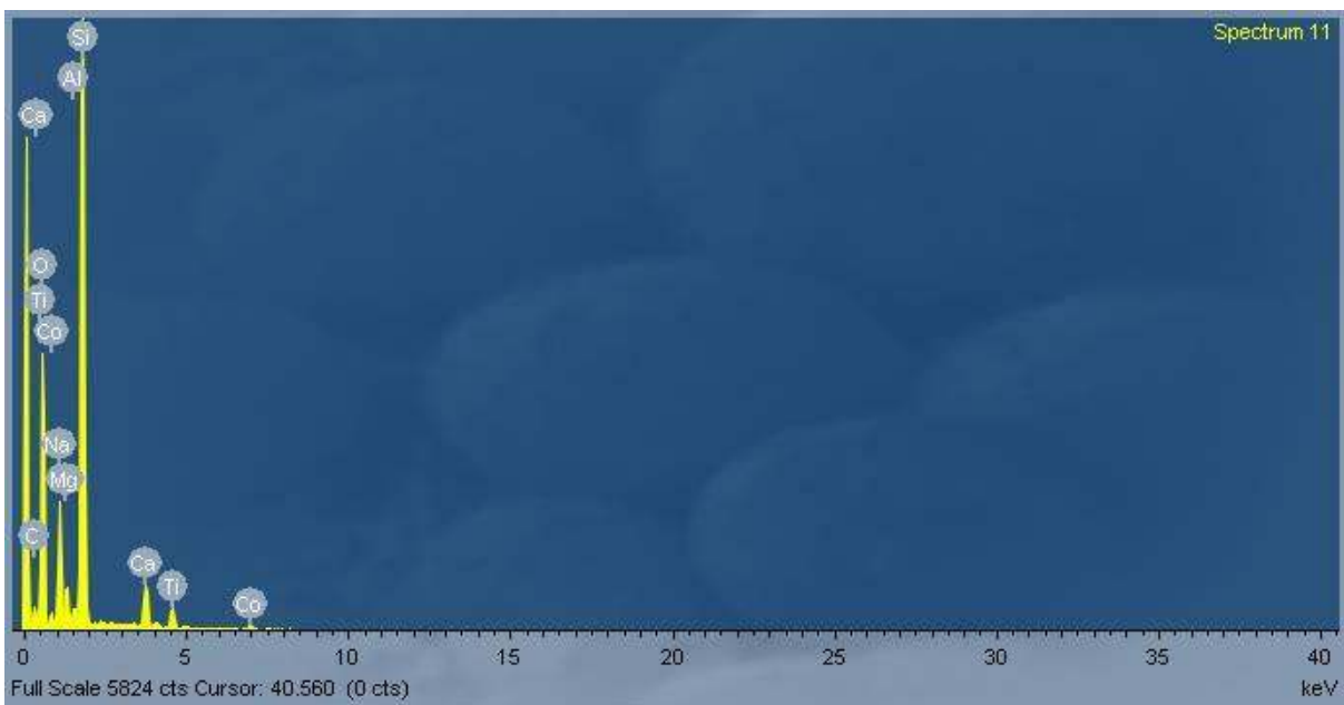
Figure 1c, EDS for TiO 2 /CoO core-shell thin film annealed at 573K
