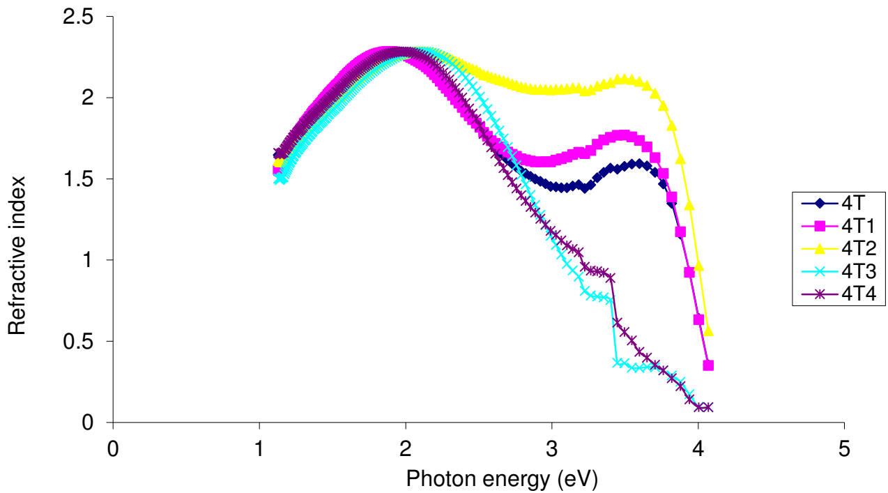
Fig. 2: Refractive index vs. photon energy for TiO 2 /CoO core-shell thin films
