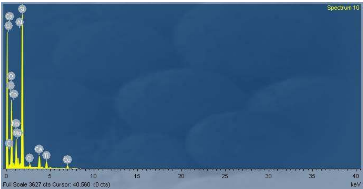
Figure 1b, EDS for TiO 2 /CoO core-shell thin film annealed at 373K
