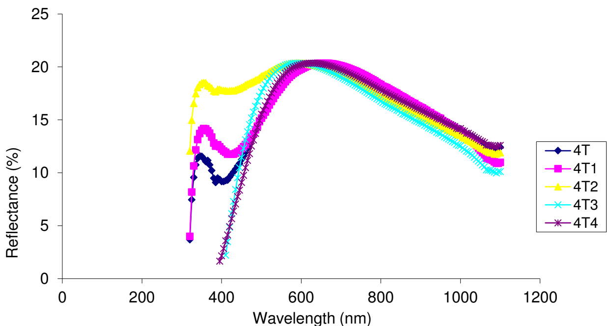
Fig. 3: Reflectance vs. wavelength for TiO 2 /CoO core-shell thin films
